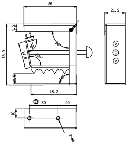
ZGP312 1&3LED mounting clip GG
