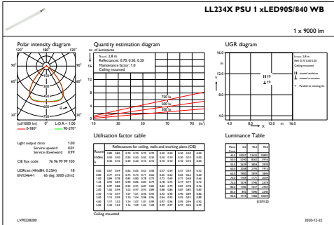
IFGU1_LL234XPSU1xLED90S840WB
