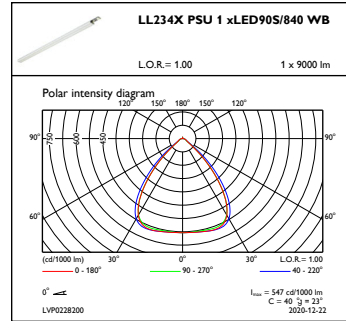
OFPCL_LL234XPSU1xLED90S840WB
